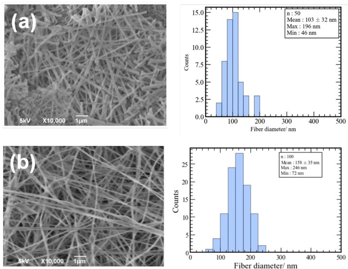
Fig.3 Typical SEM images and fiber diameter distributions of the prepared (a) SiO 2 NF xerogel sheets and (b) SiO 2 NF nonwoven sheets. Fiber diameter distribution of the SiO 2 NFs in the sheets obtained by SEM image analysis.
