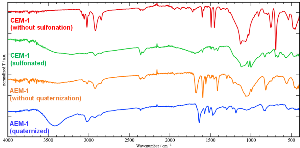
Fig.5 Typical FTIR spectra of the prepared AEM and CEM containing SiO 2 NF reinforcement.
